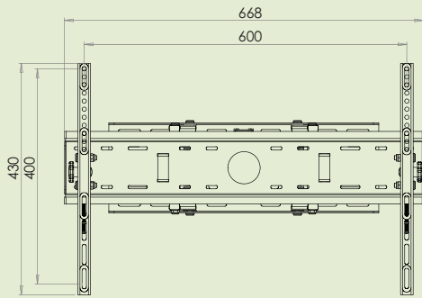
VESA Details
