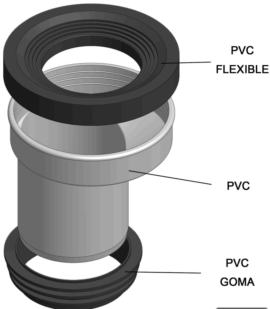
DESPIECE
