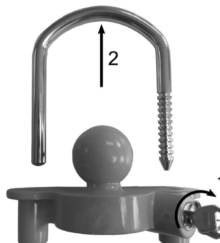
Figure 2 : retirer l'étrier
