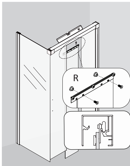
8B PLACE UPPER GUIDE TO CENTRAL SLID PANEL AND HANG UP IT.
