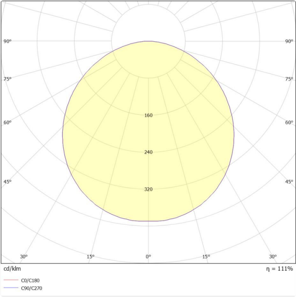
Diagrama polar DLM20SGW
