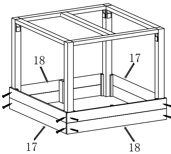
F 16PCS
