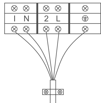
Cable clamp
