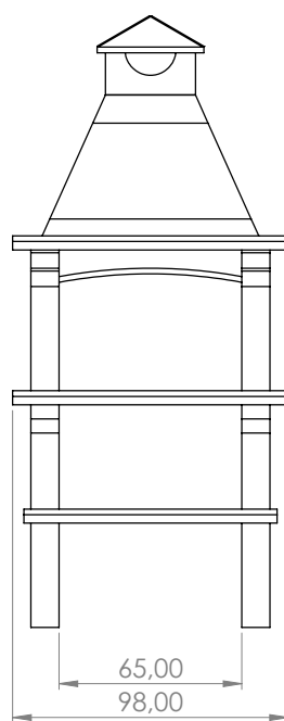
Front view
