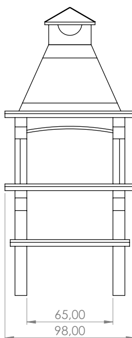
Front view
