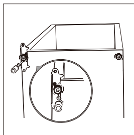
Step 7: Reassemble lower suspension and reattach height-adjustable feet.
