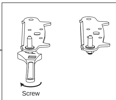
Step 5: Unscrew and remove the bottom hinge pin, turn the bracket over and replace the pin.
