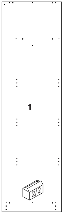
580 x 2050 mm.
