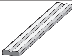
1 x L3 | 1177 x 90 x 22mm | ID 26156 1 x L4 | 1310 x 90 x 22mm | ID 26389 1 x L5 | 1810 x 90 x 22mm | ID 26112
