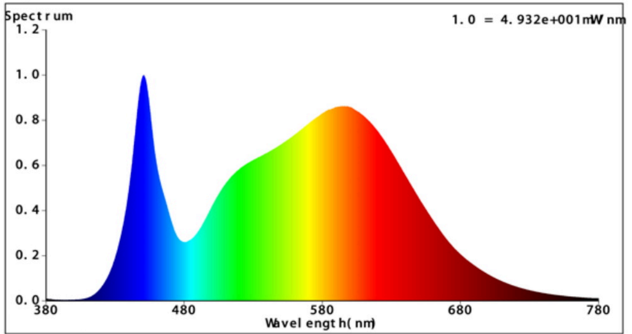
Spectral Distribution
