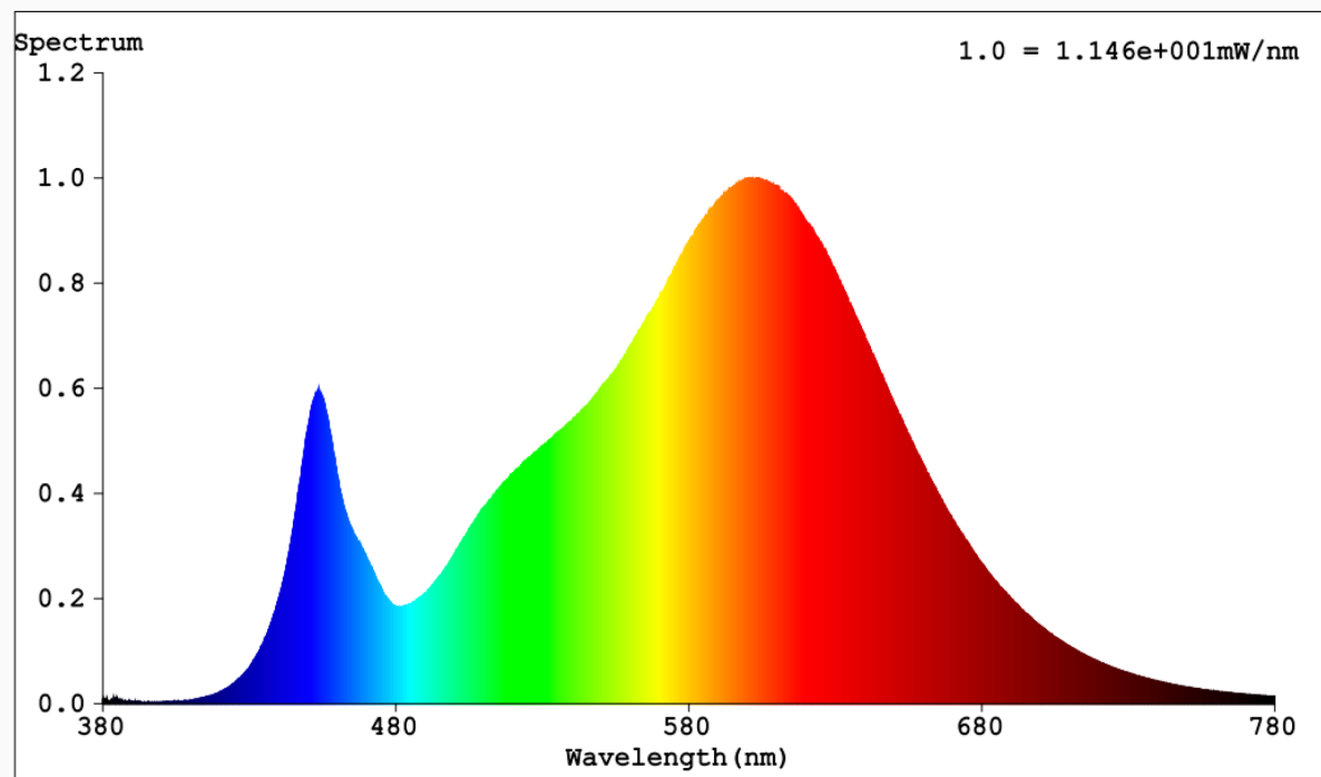
Data 3: Spectral power distribution for light source of FY-XF-1047-641,78MM-2835-12B2C:
