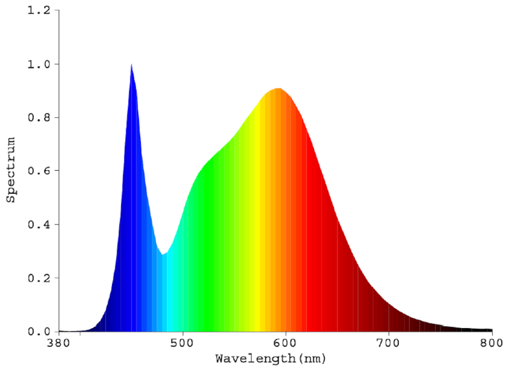
Spectral power distribution for light source of PCB1172X10-CCT-60W-2835 CC 4000K:
