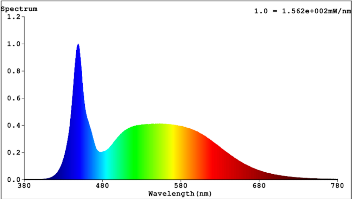
Spectral power distribution for light source of PCB777x10-D-15W-2835 6500K:
