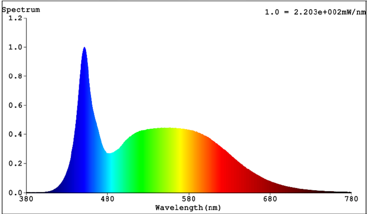
Spectral power distribution for light source of PCB572x10-D-15W-2835 6500K:
