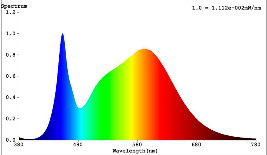
Data 3: Spectral power distribution for light source of P6252-BMHU-NW7h:
